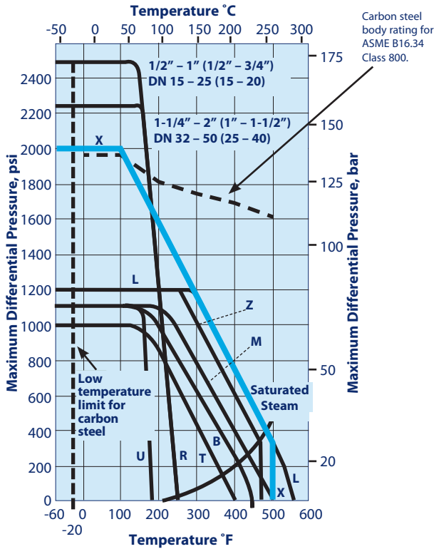
1/2" – 2" (DN 15-50) Standard Port, 1/2" – 1-1/2" (DN 15-40) Full Port Valves
